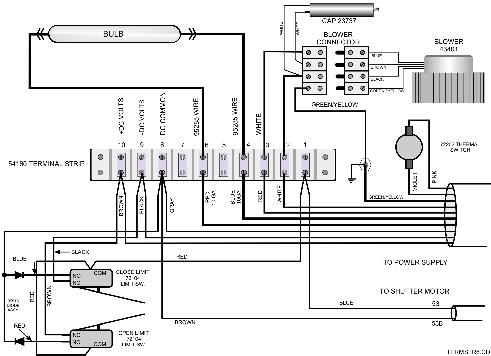
TYPICAL VIOLUX / MULTI LAMPHEAD WIRING - 3 WIRE BLOWERS (NOT COUNTING GROUND)
